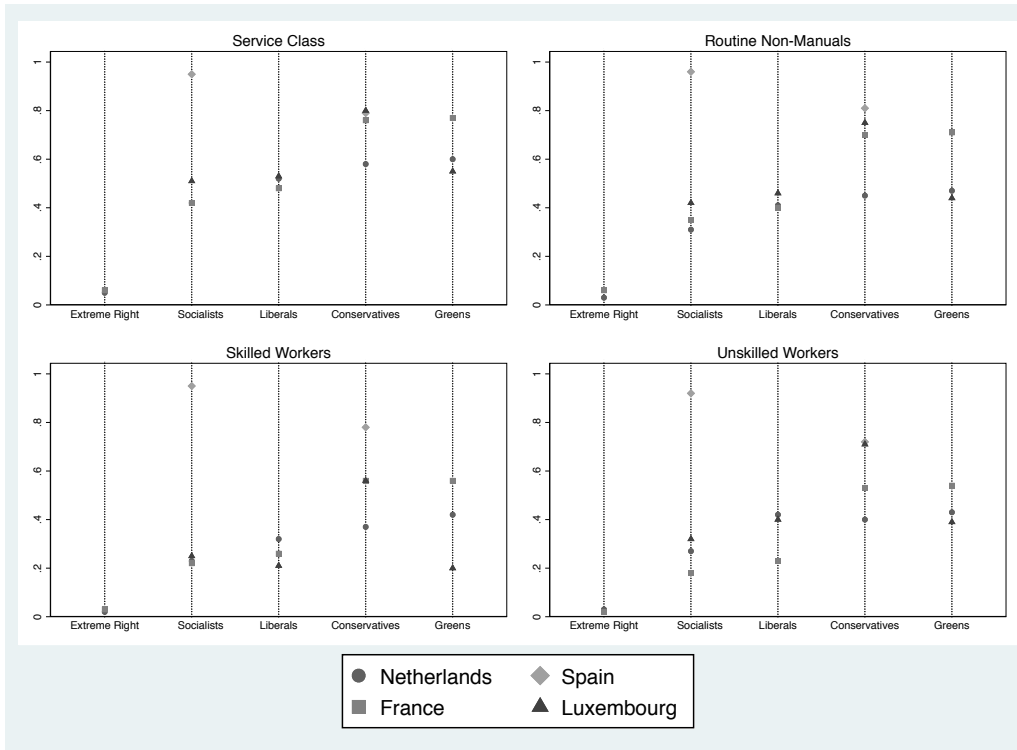
Figure 1a: Predicted Probabilities of voting in favour of the TCE depending on party support I (social class held constant)
